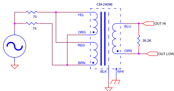
TEST CIRCUIT 2 - Parallel
