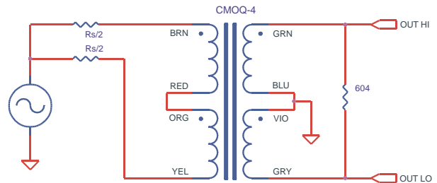
TEST CIRCUIT 2
