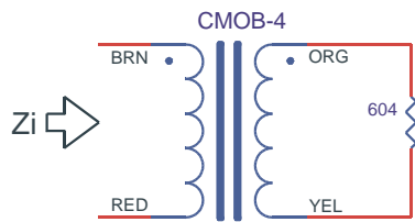
TEST CIRCUIT 3
