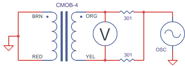
TEST CIRCUIT 2
