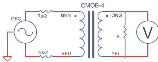
TEST CIRCUIT 1
